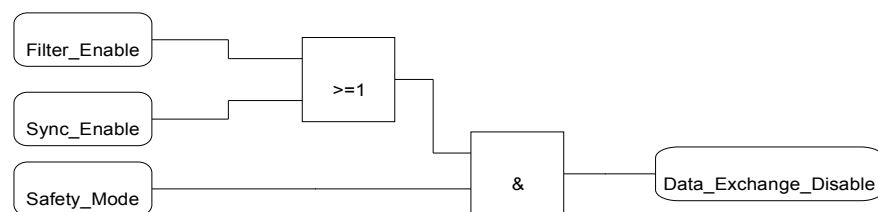
Figure 16: Flowchart - Data_Exchange_Disable
