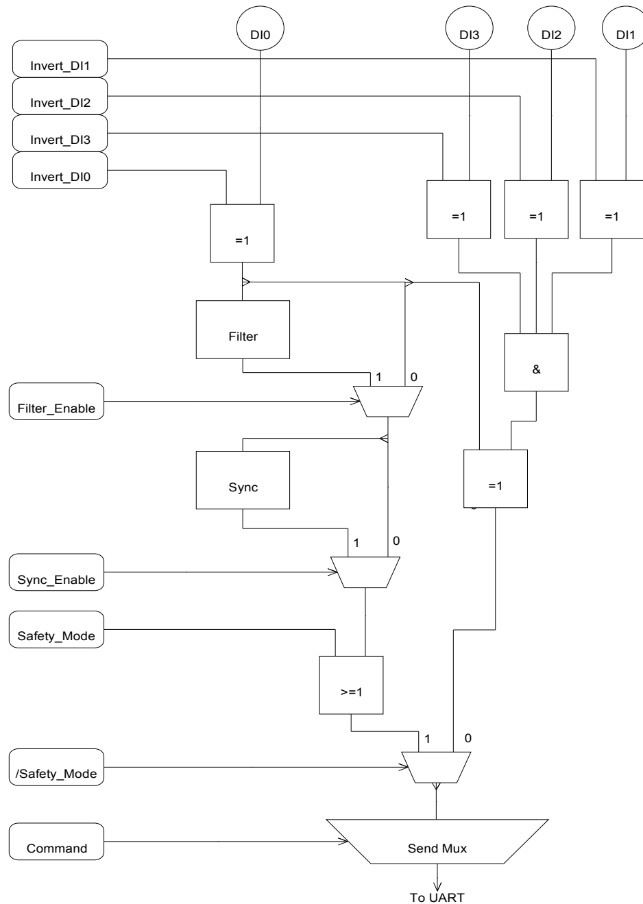
Figure 15: Flowchart - Input D0 in Safety Mode
