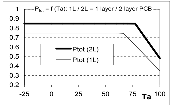
Figure 1: P_{tot} = f(\theta_a)
